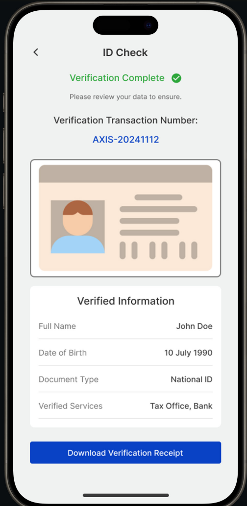
Verification Screen
