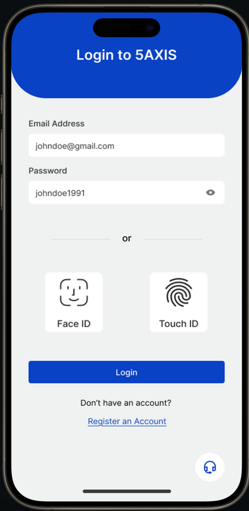
Account Creation
