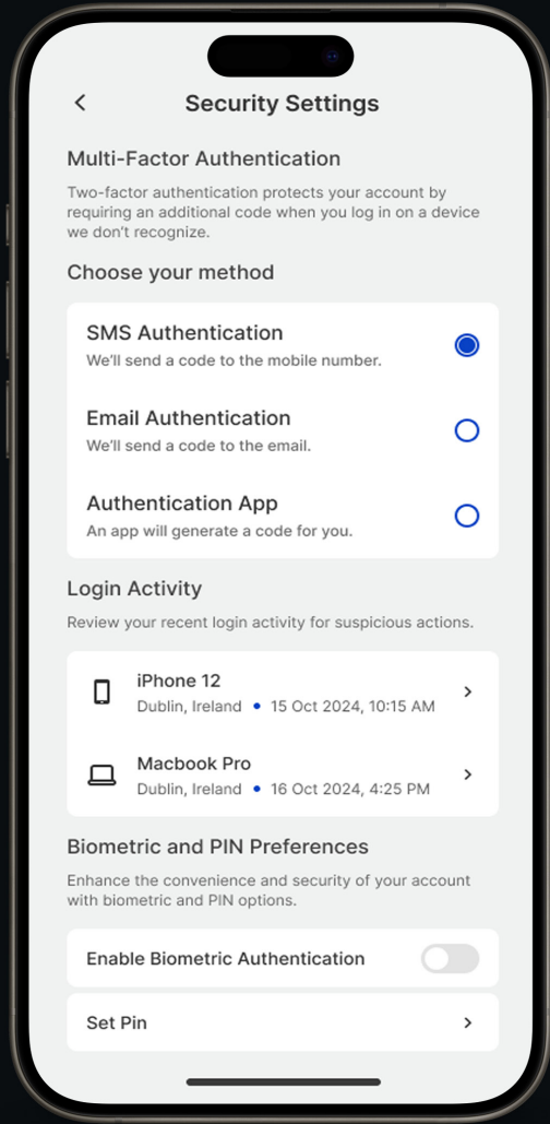
Security Settings
