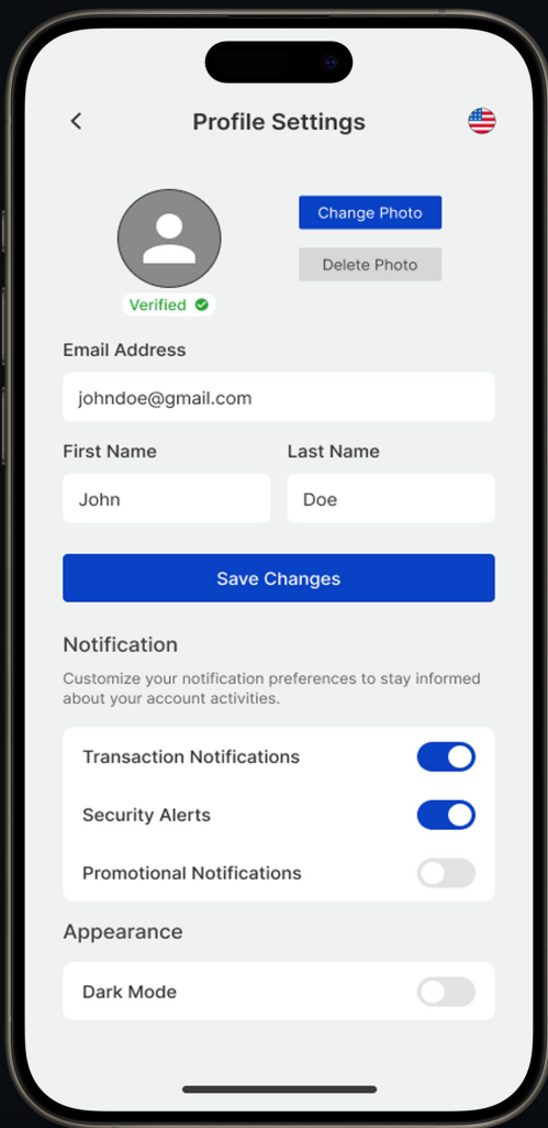
Profile Settings
